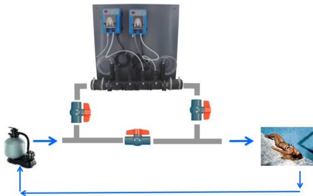
Installation in bypass configuration
